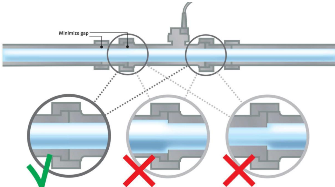
Fig 6.2 Flow Sensor Mechanical Installation – Avoid changes in bore diameter
